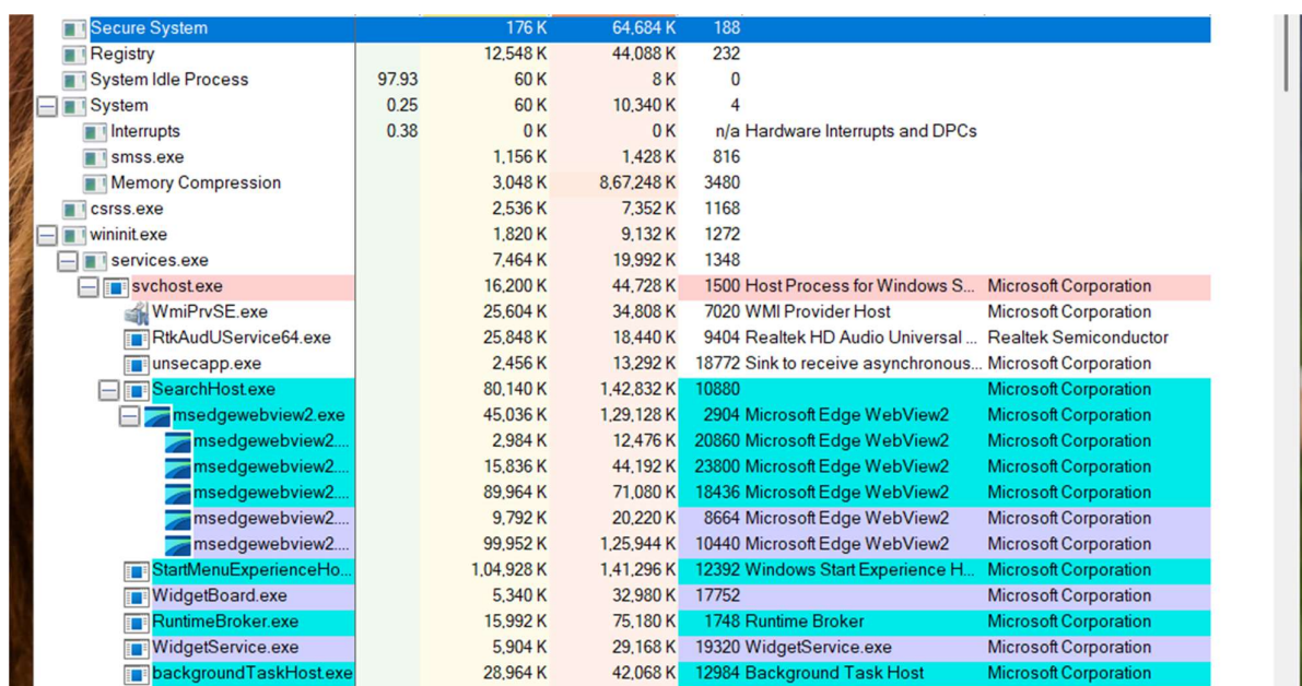
Figure 2: Process Explorer dashboard displaying hierarchical process trees and resource metrics
