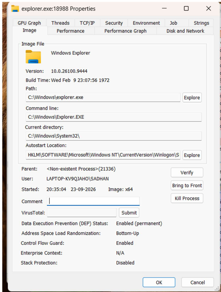
Figure 3: Inspecting image properties, cryptographic signatures, and execution file paths
